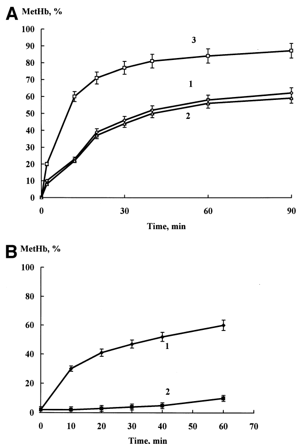
Fig. 4. The time course of intracellular methHb formation (A) after RBCs exposure to 1 mM (1, 2) and 4 mM NaNO 2 (3) and (B) after RBC exposure to 4 mM K 2 Cr 2 O 7 (1, 2), PBS, pH 7.4, 37°C. Erythrocytes were treated with oxidative agents before (1, 3) or after (2) preliminary cell modification by 1 mM DIDS.
